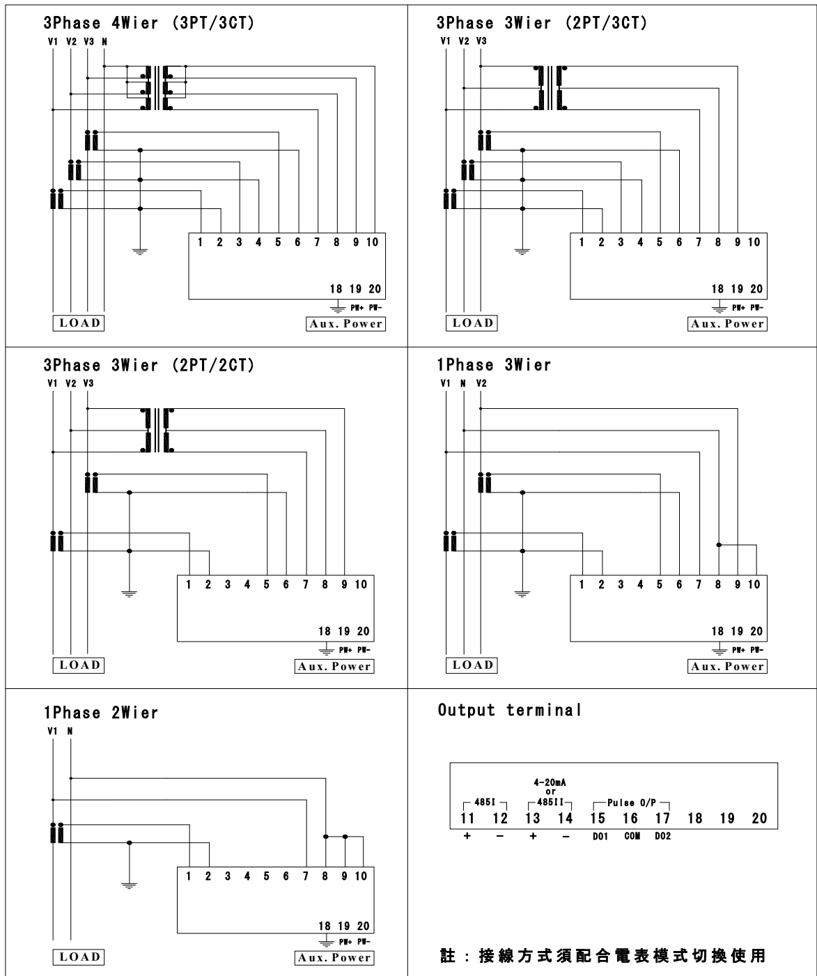
Connection Diagram Model :TDPF
